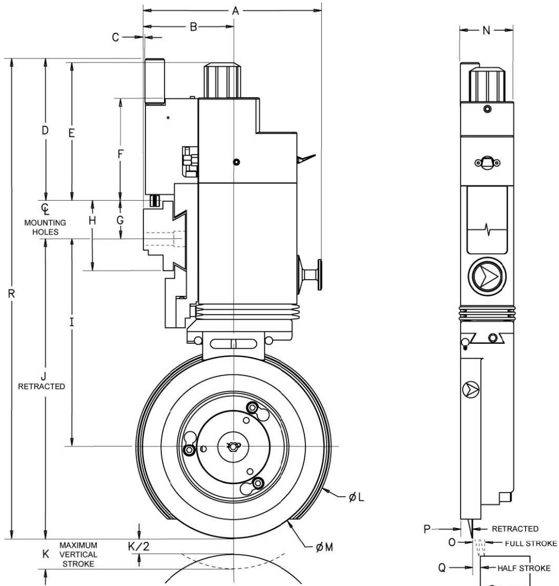
Performance Series Manual Class I Knifeholder with Rigid Blade Cartridge Dimensions
